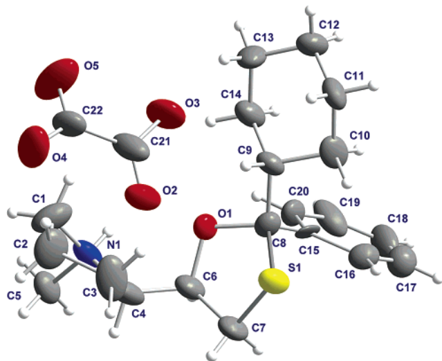
Figure 1. Thermal ellipsoid plot (50% ellipsoids) of compound (-)-2 oxalate.
